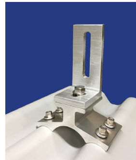
POWMOUNT PMR1-S
