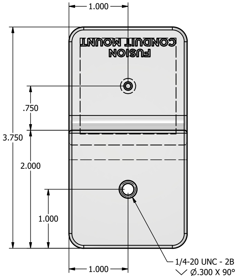
TOP VIEW
