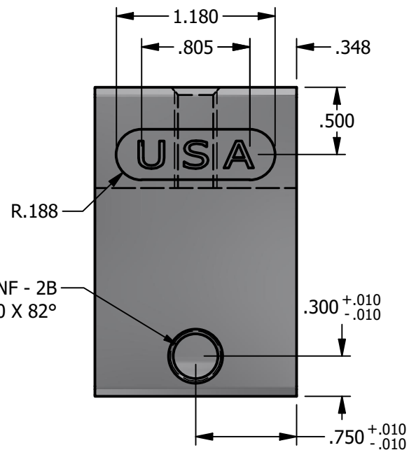
RIGHT VIEW
