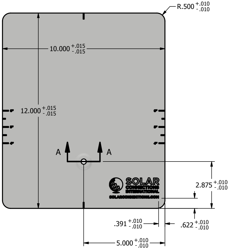
TOP VIEW
