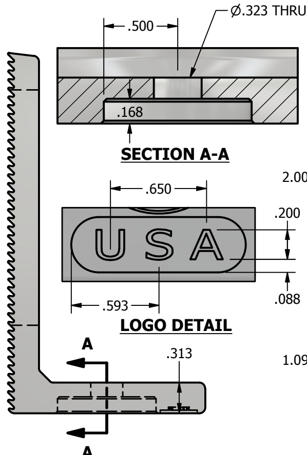
RIGHT VIEW
