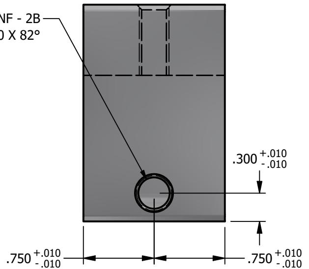
RIGHT VIEW
