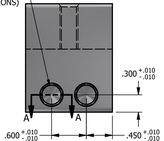
RIGHT VIEW
