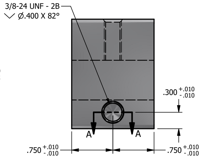
RIGHT VIEW
