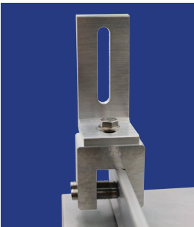
PV CUBE
