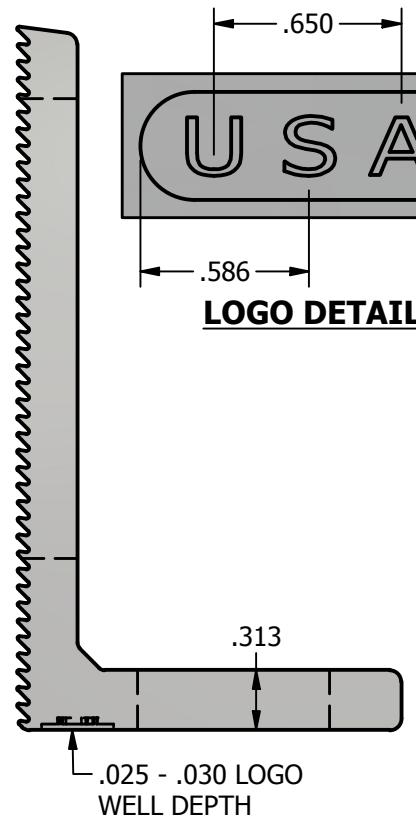
RIGHT VIEW
