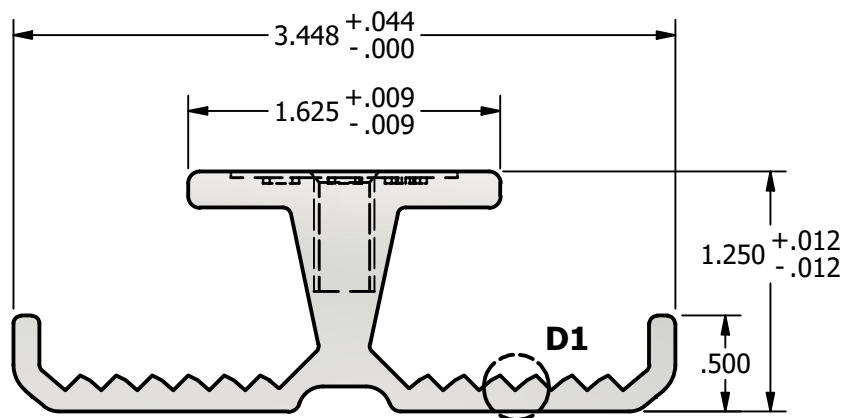
PROFILE VIEW
